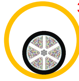
Slotted core cable with partially bonded ribbon 288C OD : 17mm
