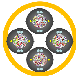
SWR/WTC 4 x 288C = 1152C
